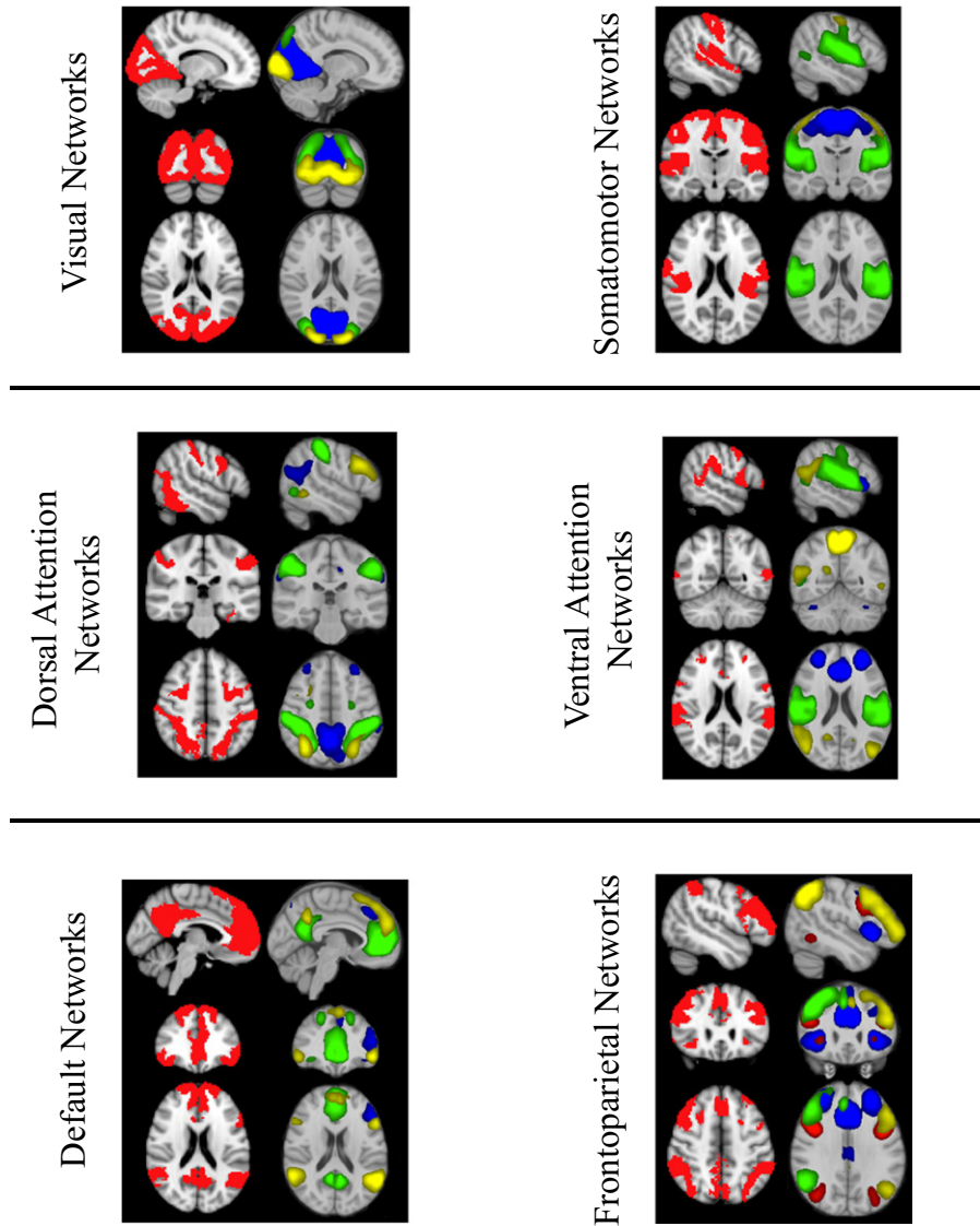
Fig. 3. Resting state networks from the current study compared to reference networks (Yeo et al., 2011). Reference networks are plotted on the left in red. RSNs from the current study were spatially combined into a single image and plotted in contrasting colors.
