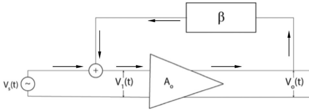
Fig. 1. A simple operational amplifier with a time delay \tau in feedback circuit \beta .
