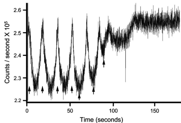
Fig. 3. Flavoprotein redox oscillations are inhibited by pulsed magnetic fields timed to coincide with minimal flavoprotein auto fluorescence, and they amplify oscillations when timed at minimums [Rosenspire et al., 2005, Fig. 11].
