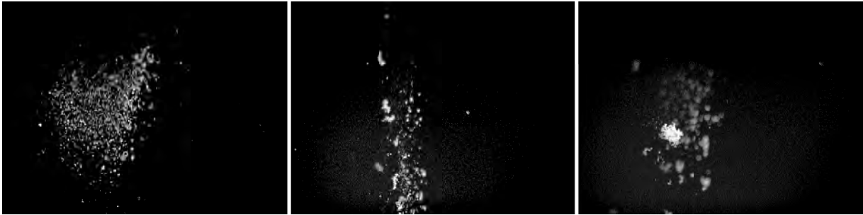
Figure 3: Growth of agglomerates during cloud squeezing by CMS. The horizontal image size is 10 mm with 0.5 s between the frames .
