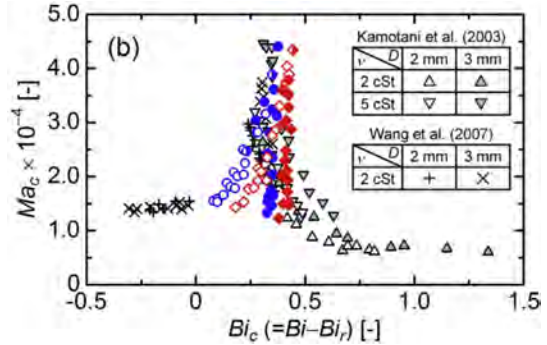
Figure 2: Critical Marangoni number ( Ma_c ) for the onset of instability plotted as a function of Biot number, Bi . Blue markers depict Prandtl number Pr = 28 and red diamonds Pr = 67 .
