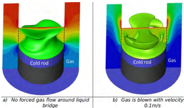
Figure 4: Computed temperature field in liquid bridge filled with n-decane and air as gas; \Delta T = 7.4K , T_{\text{mean}} = 298K and T_{\text{gas}} = 293K . Iso-surfaces of the mean temperature inside the liquid are shown by green colours. The temperature field in gas phase is illustrated by colors.
