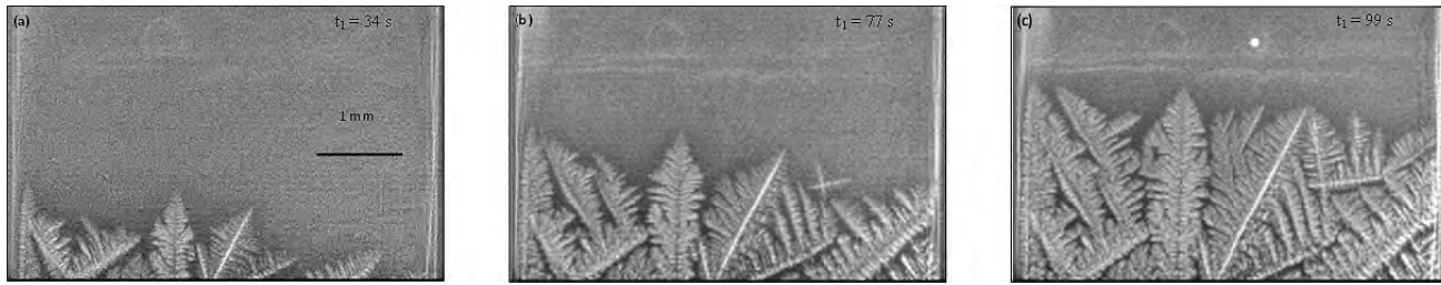
Figure 2: Sequence of three radiographs illustrating the columnar solidification of Al-20wt% Cu in microgravity conditions (MASER-12 experiment), with a temperature gradient of about 150 K/cm and a cooling rate of 0.15 K/s on both heaters.
