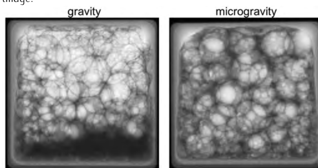
X-ray images of metal foam.
