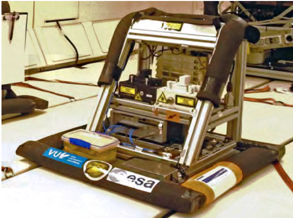
Figure 3: Bio-X Experiment, two lensless microscopes (black and white) and a box with samples.
