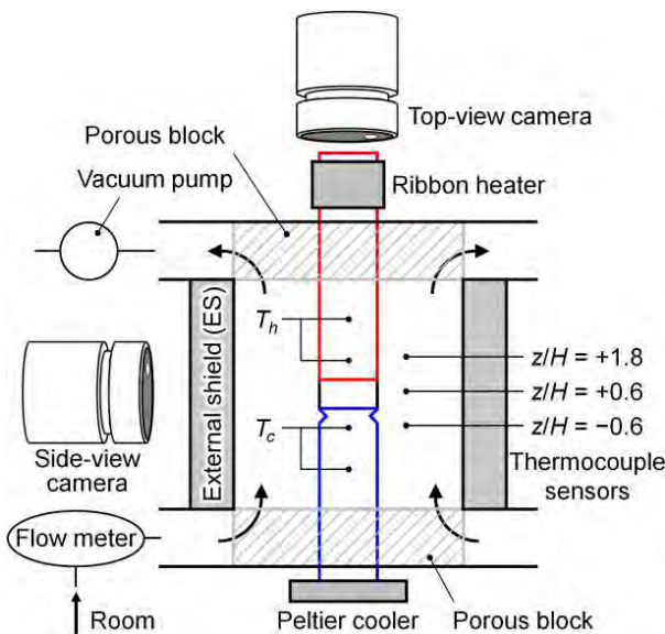
Figure 1: Experimental set-up to study the convective heat transfer effect on the instability in a liquid bridge.
