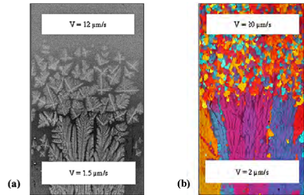
Figure 1: Columnar-Equiaxed Transition obtained by an increase of the growth velocity during the directional solidification of a refined Al - 3.5 wt% Ni. The real width of the two images is 6 mm. (a) In situ X-ray radiograph recorded at ESRF (European Synchrotron Radiation Facility). (b) Optical microscopy image obtained after a post-mortem metallography of the sample.
