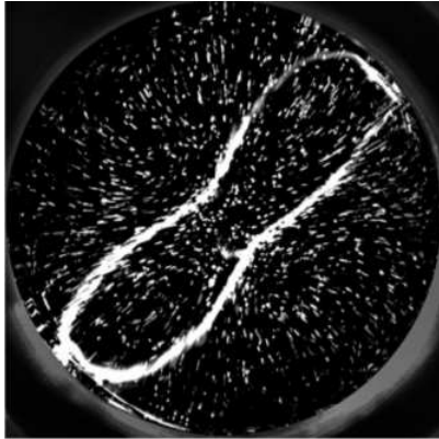
Figure 7: Experimental observation. A top-view through a transparent upper disk of particles distribution (seen as white specs) in a liquid bridge with a cylindrical interface.
