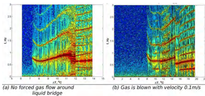
Figure 5: Experimental Fourier map. The experiment starts from \Delta T below critical value and then temperatures difference gradually increases. For each given \Delta T the Fourier spectrum is built and then they are combined in a map presented here. T_{\text{mean}} = 298K and T_{\text{gas}} = 293K
