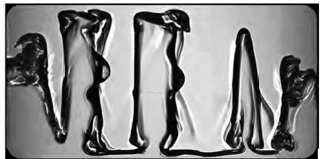
Figure 2: Interfacial patterns in miscible liquids under vibrations parallel to initially horizontal interface at f=8\text{Hz} , A=10.7\text{mm} . (left: on ground; right: in microgravity)
