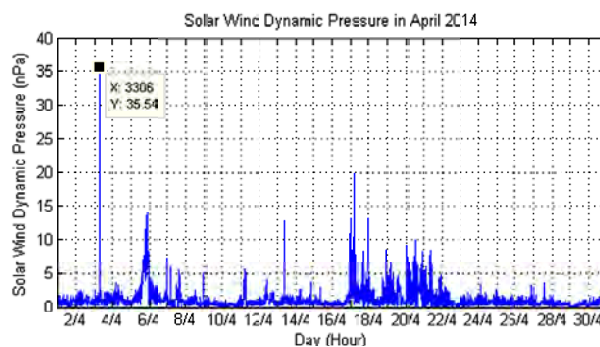
Figure 2: Solar wind pressure (April 2014).
