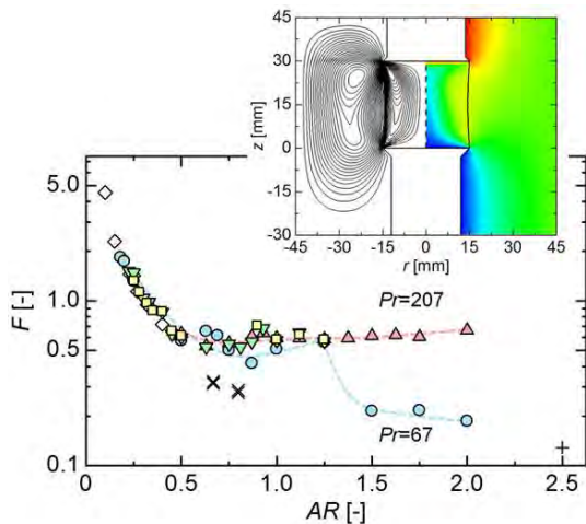
Figure 3: Dimensionless frequency ( F ) detected at the onset of oscillation in liquid bridges of high Prandtl number liquids experimented in microgravity environment on the ISS.
