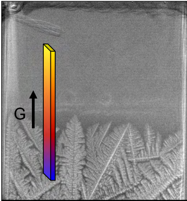
X-ray image of solidification in microgravity of Al 20 wt %Cu, temperature gradient indicated.
