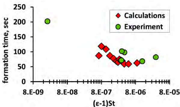
Figure 9: Comparison between results of the computer modelling and of the experiments. Formation time of coherent structures is plotted versus inertia of heavy particles, which is (\epsilon - 1)St , where \epsilon is the particles to liquid density ratio, and St is the Stokes number – the ratio of the characteristic time of a particle to a characteristic time of the flow.
