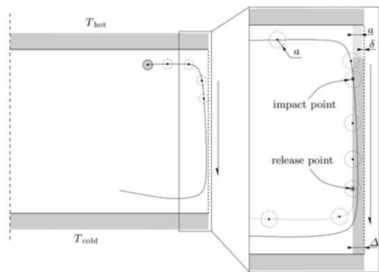
Figure 10: Sketch of the theoretical model applied to a spherical particle in an axisymmetric liquid bridge. The full line represents the trajectory if particle–boundary model is enforced, whereas the dotted line shows the trajectory if the collision between particles and free-surface is theoretically modelled.
