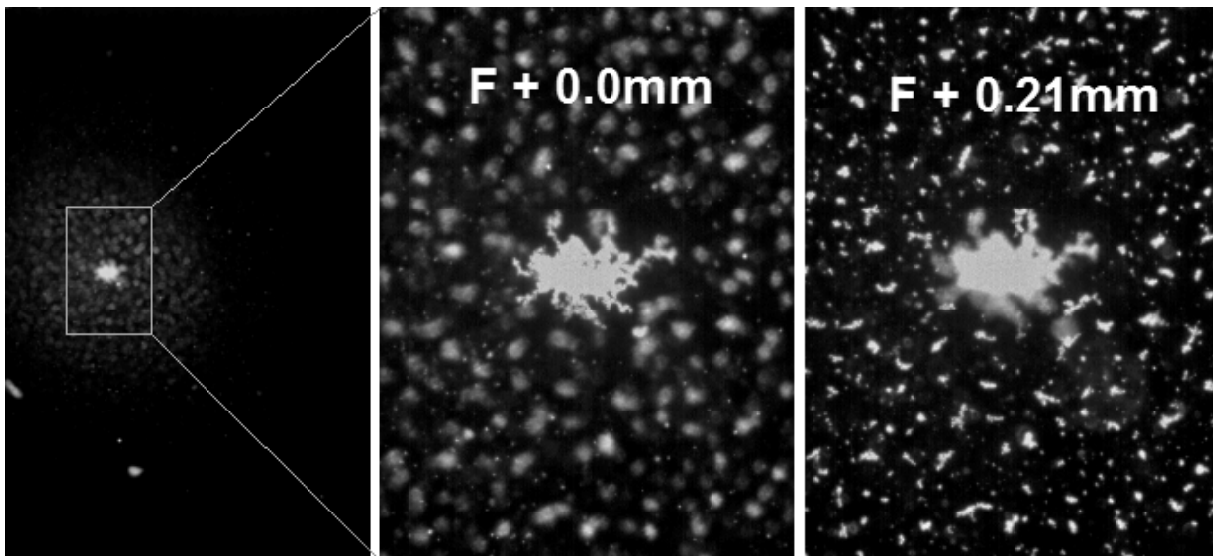
Figure 2: Agglomerates being delivered to the focal plane of the observation camera and being scanned through the camera's field of view. The horizontal size is 8.6 on the first and 1.8 mm on the last two images.
