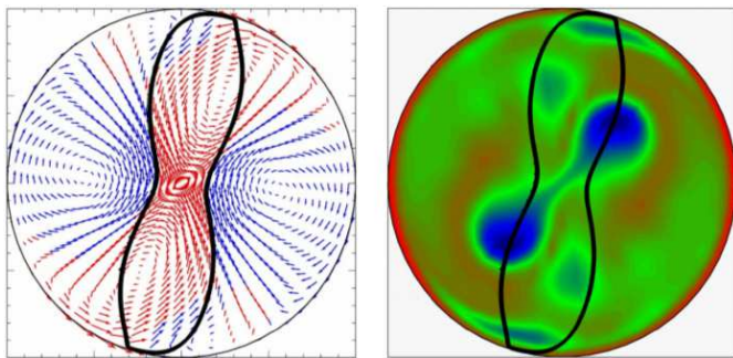
Figure 8: Computer modelling of the experiments. Top view of particles distribution (seen as black symbols) in a liquid bridge. The particles form a stable symmetric coherent structure whose correlations with velocity (temperature field) are shown on the left (right) panel.
