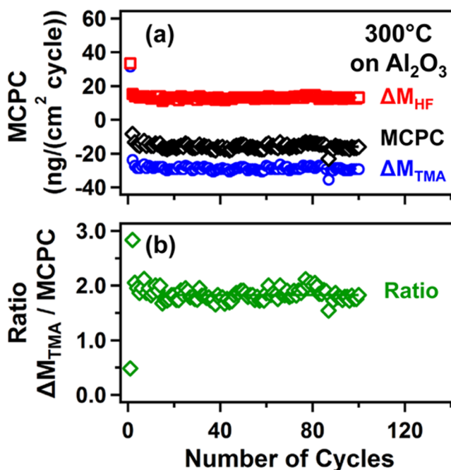
Figure 3. (a) Mass change after the TMA exposure ( \Delta M_{\text{TMA}} ), mass change after the HF exposure ( \Delta M_{\text{HF}} ) and mass change per cycle (MCPC) versus number of ALE cycles at 300 °C. (b) \Delta M_{\text{TMA}}/\text{MCPC} ratio versus number of ALE cycles.
