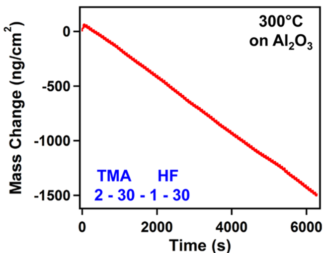
Figure 1. Mass change versus time for \text{Al}_2\text{O}_3 ALE using sequential TMA and HF exposures at 300 °C.
