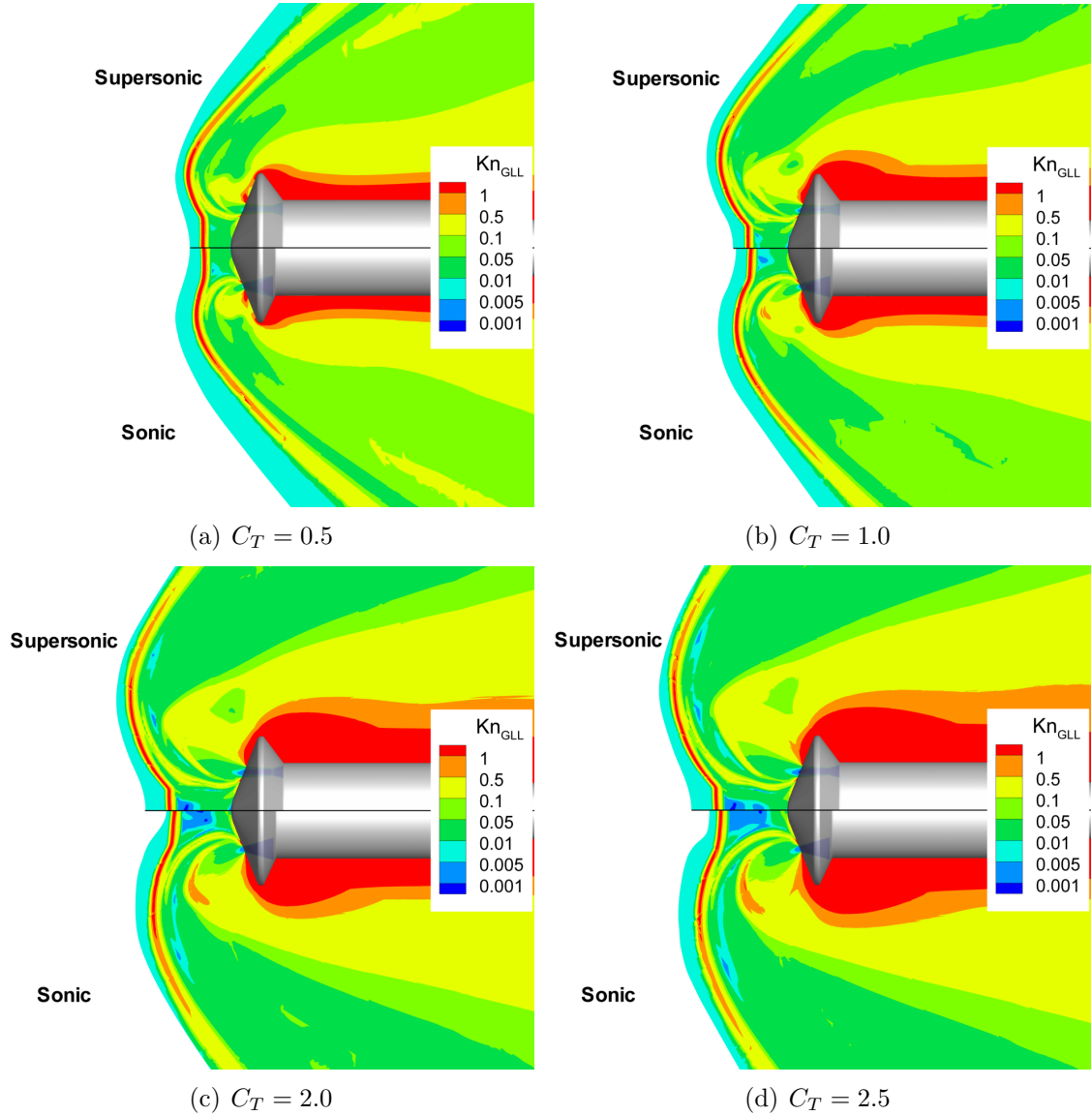
Figure 4.8: Comparison of gradient-length local Knudsen number contours for sonic (bottom) and supersonic (top) peripheral PD jets at various thrust coefficients.
