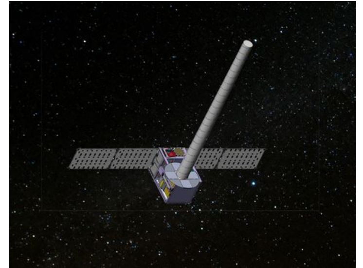
Rendering of a helical L-band antenna redwirespace.com/newsroom/roccor-creates-helical-l-band-antenna/?rdws=nnn.xffxcv.tfd&rdwj=3094 1
