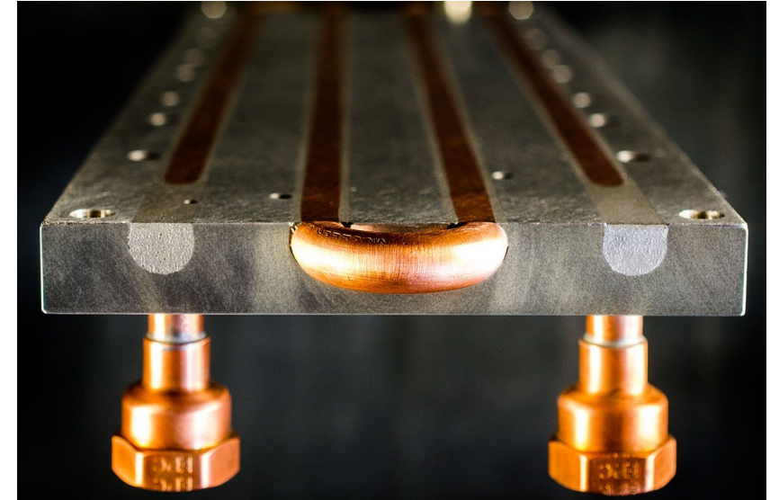
EMP Cooling Coil for Thermal Management electromechanicalproducts.com/thermal-management/
